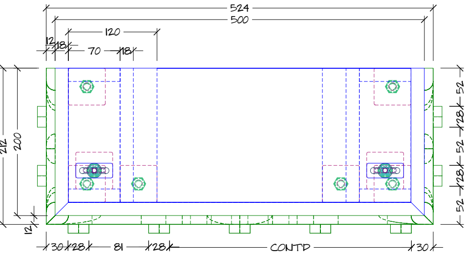
C.1 PLAN VIEW 1:5@A3
