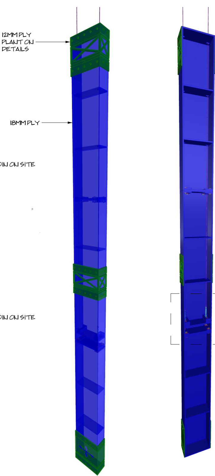
C.1 3D VIEWS NA@A3
