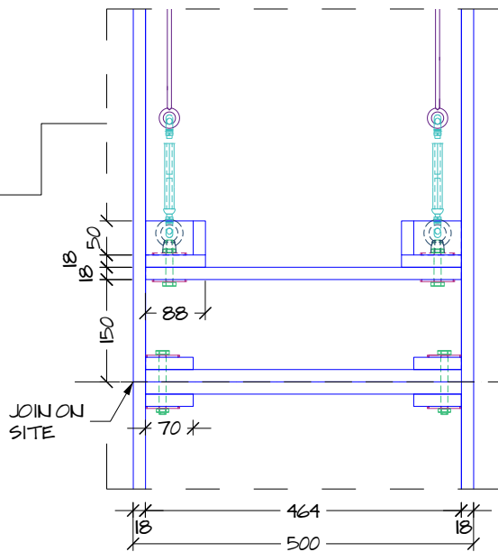
C.1 REAR VIEW 1:10A3
